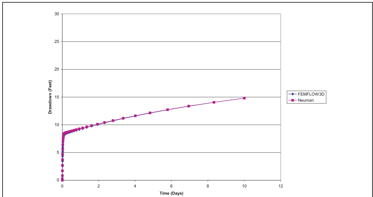
Figure 4-15 Comparison of FEMFLOW3D Simulated Drawdowns With Neuman Solution for Deep Well at a Distance of 400 Feet From Pumping Well
