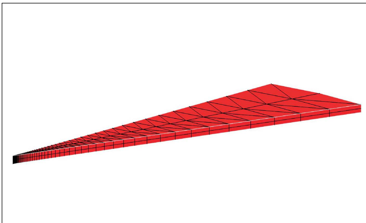
Figure 4-1 Finite-Element Mesh Used for Theis Model Simulation
