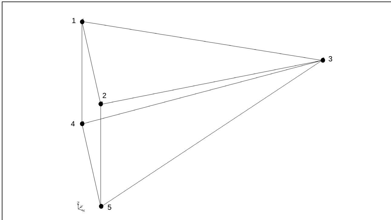
Figure 1-4 Wedge-Shaped Element With One Zero-Height Edge
