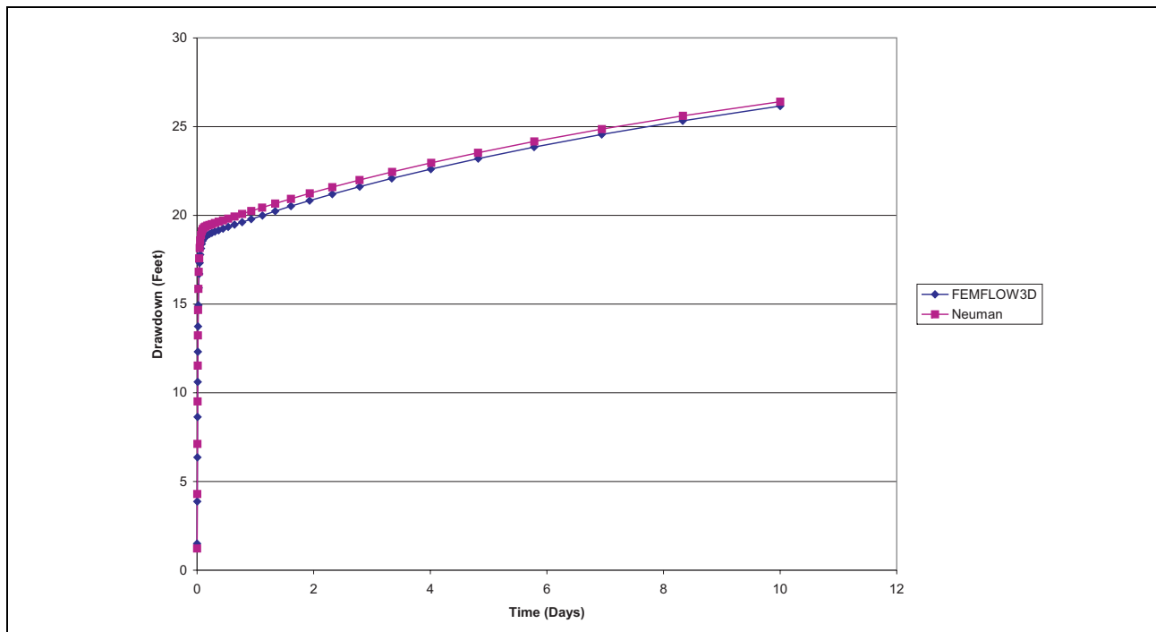
Figure 4-12 Comparison of FEMFLOW3D Simulated Drawdowns With Neuman Solution for Deep Well at a Distance of 200 Feet From Pumping Well
