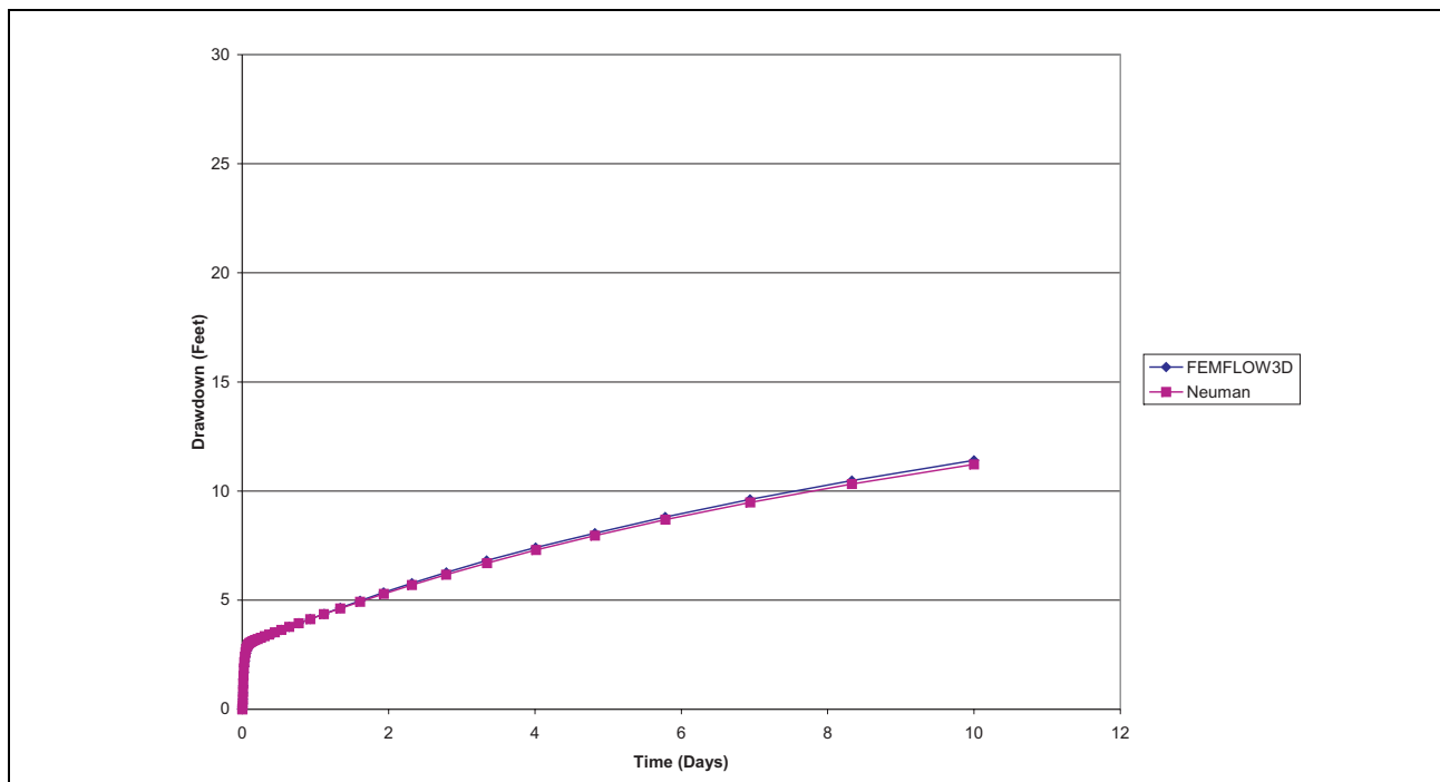
Figure 4-13 Comparison of FEMFLOW3D Simulated Drawdowns With Neuman Solution for Shallow Well at a Distance of 400 Feet From Pumping Well
