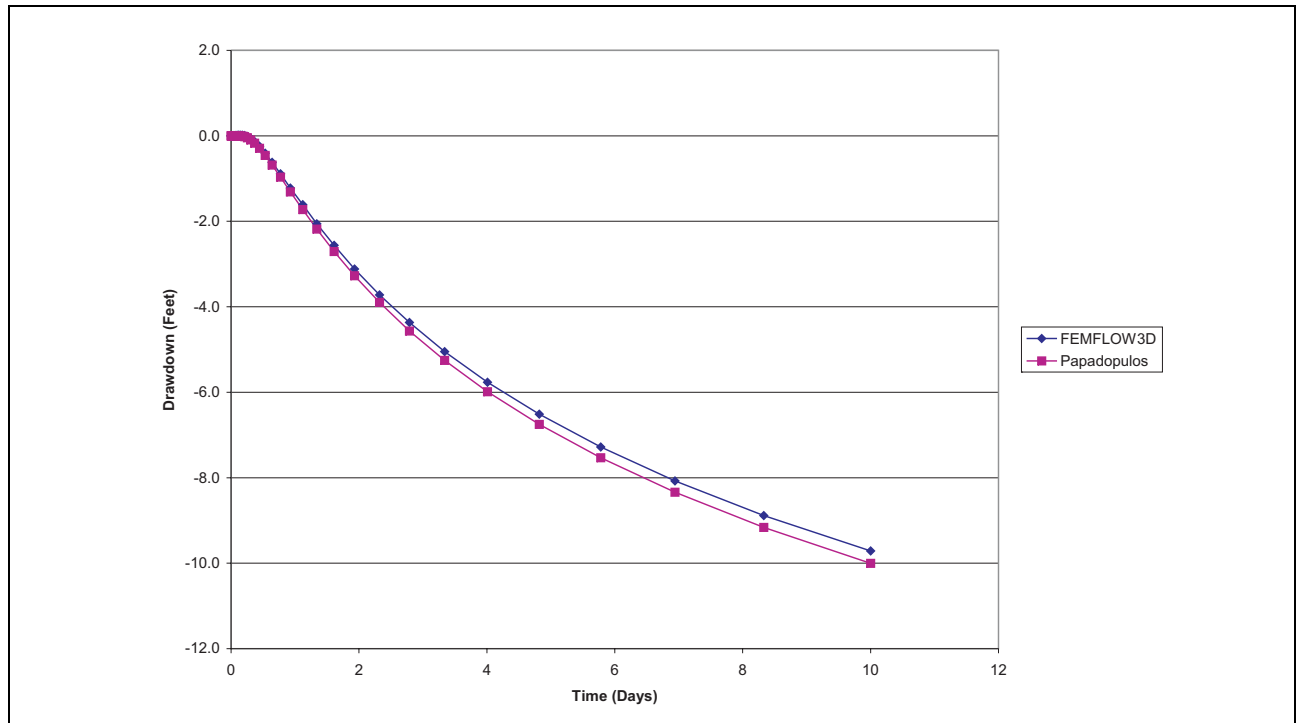
Figure 4-7 Comparison of FEMFLOW3D Simulated Drawdowns With Papadopoulos Solution at a Distance of 409 Feet From Pumping Well
