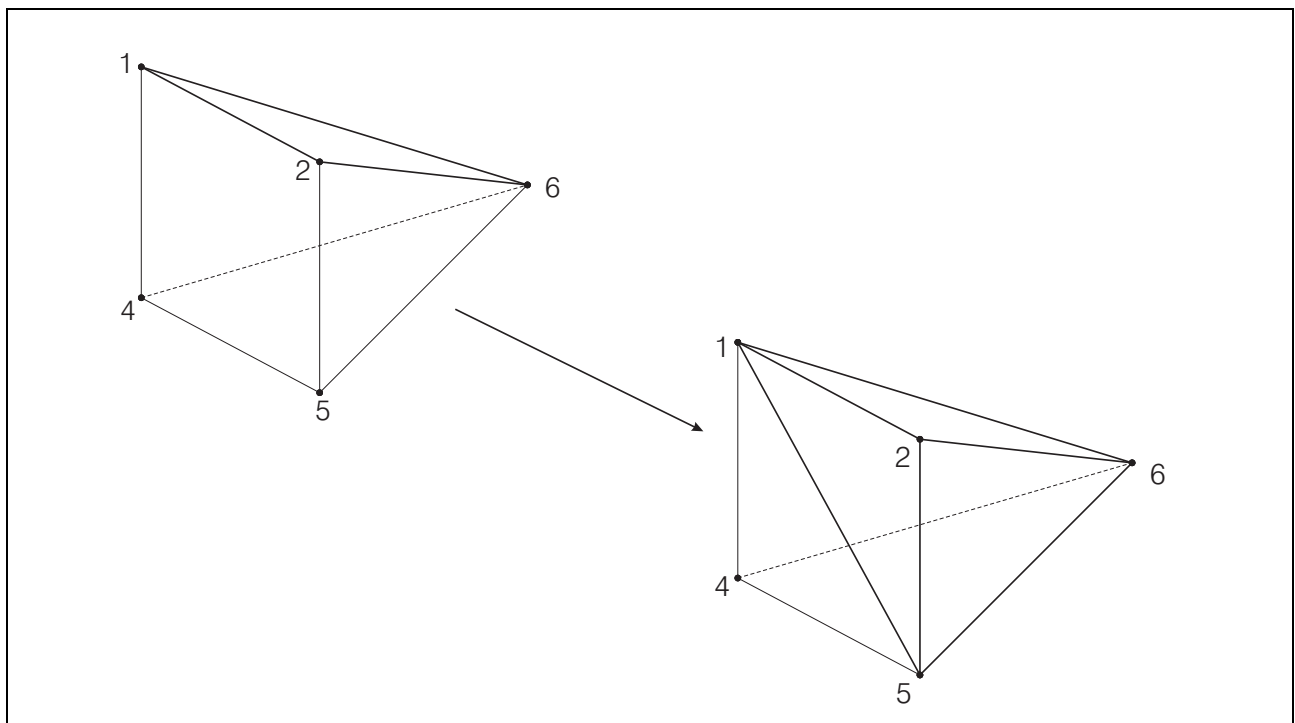
Figure 2-3 Disaggregation of Pyramid-Shaped Element Into Two Tetrahedrons
