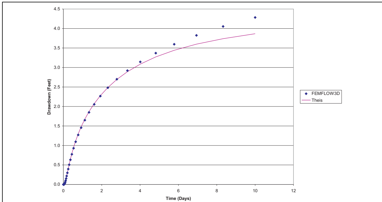
Figure 4-2 Comparison of FEMFLOW3D Simulated Drawdowns With Theis Solution at a Distance of 200 Feet From Pumping Well
