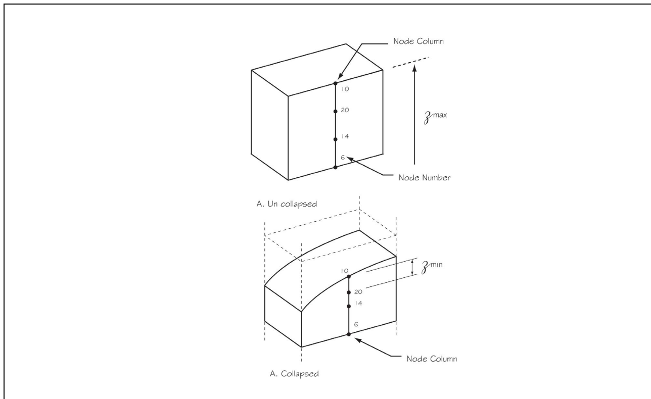
Figure 3-1 Collapsing Mesh Diagram
