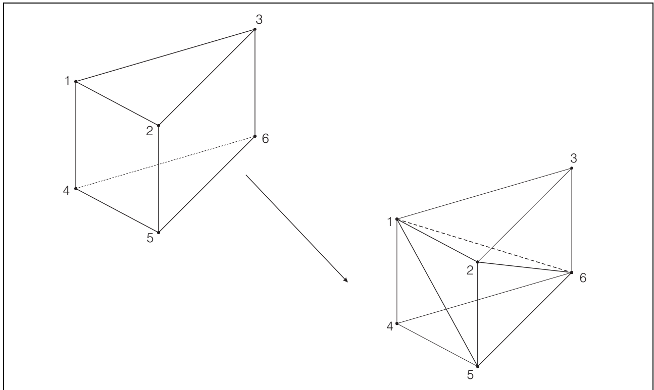
Figure 2-2 Disaggregation of Wedge-Shaped Element Into Three Tetrahedrons
