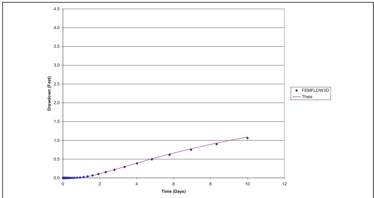
Figure 4-4 Comparison of FEMFLOW3D Simulated Drawdowns With Theis Solution at a Distance of 800 Feet From Pumping Well
