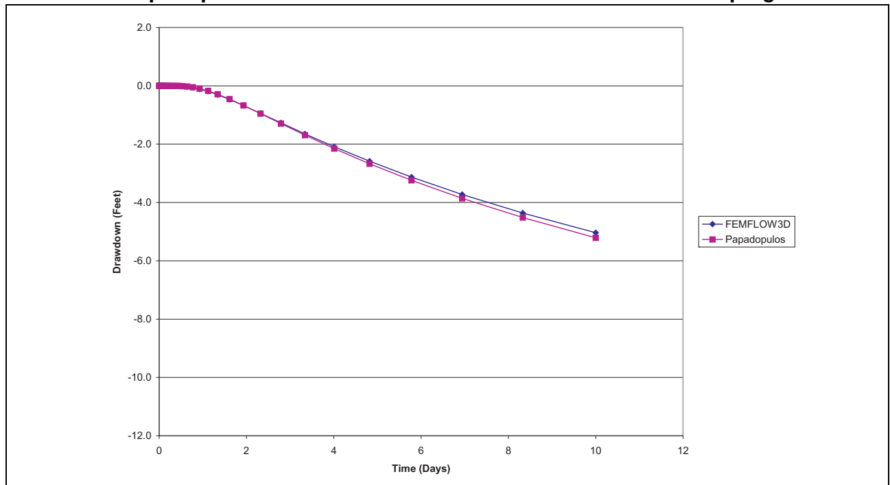
Figure 4-8 Comparison of FEMFLOW3D Simulated Drawdowns With Papadopoulos Solution at a Distance of 448 Feet From Pumping Well
