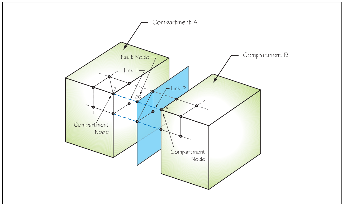
Figure 3-3 Layout for Fault Links
