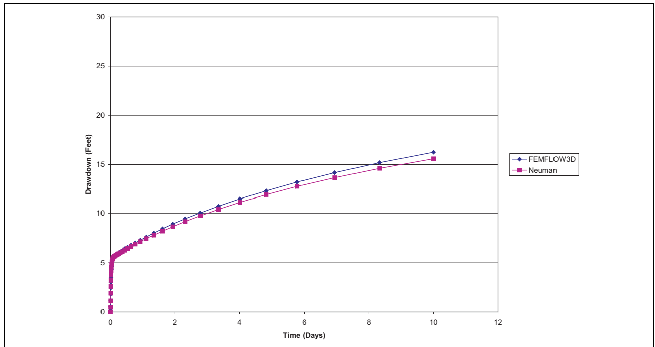
Figure 4-10 Comparison of FEMFLOW3D Simulated Drawdowns With Neuman Solution for Shallow Well at a Distance of 200 Feet From Pumping Well
