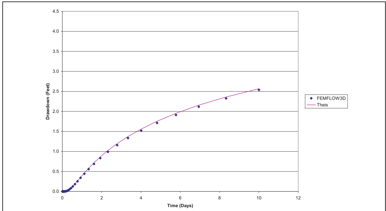
Figure 4-3 Comparison of FEMFLOW3D Simulated Drawdowns With Theis Solution at a Distance of 400 Feet From Pumping Well
