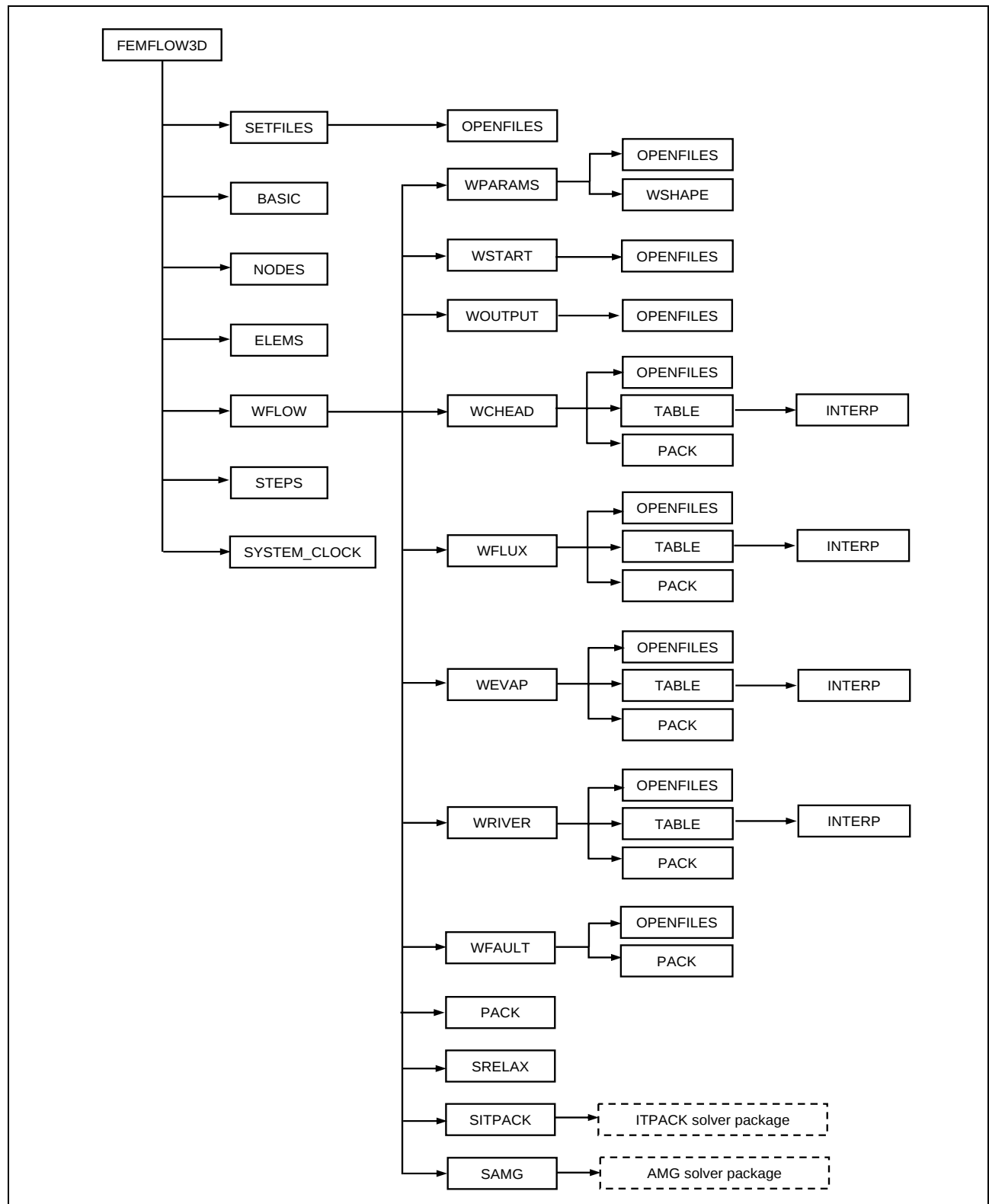
Figure 1-1 Subroutines and Functions Used in FEMFLOW3D
