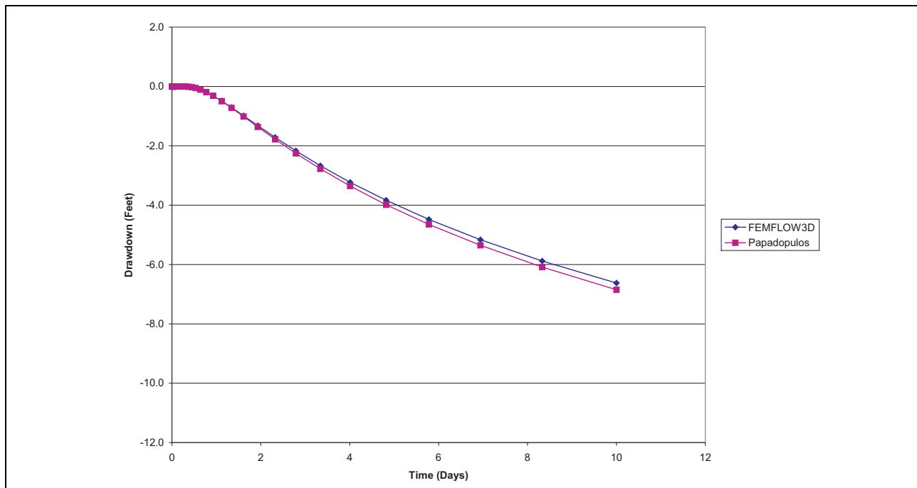
Figure 4-6 Comparison of FEMFLOW3D Simulated Drawdowns With Papadopoulos Solution at a Distance of 184 Feet From Pumping Well
