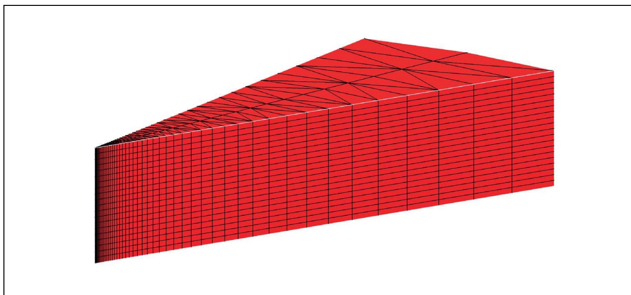
Figure 4-9 Finite-Element Mesh Used for Neuman Model Simulation
