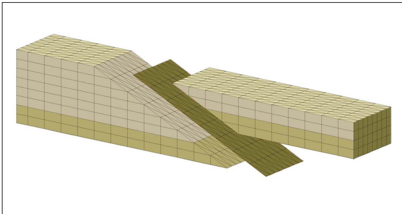
Figure 1-7 Two Hydrogeologic Compartments Offset by a Sloping Fault
