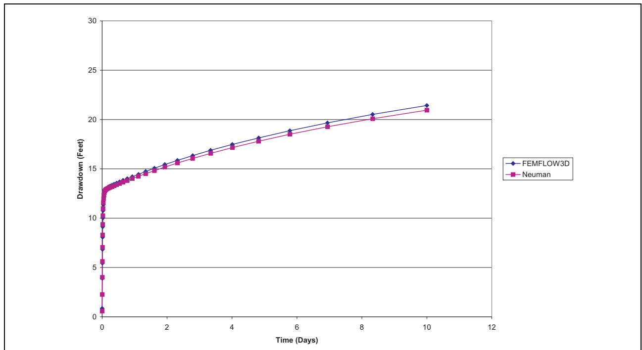
Figure 4-11 Comparison of FEMFLOW3D Simulated Drawdowns With Neuman Solution for Middle Well at a Distance of 200 Feet From Pumping Well
