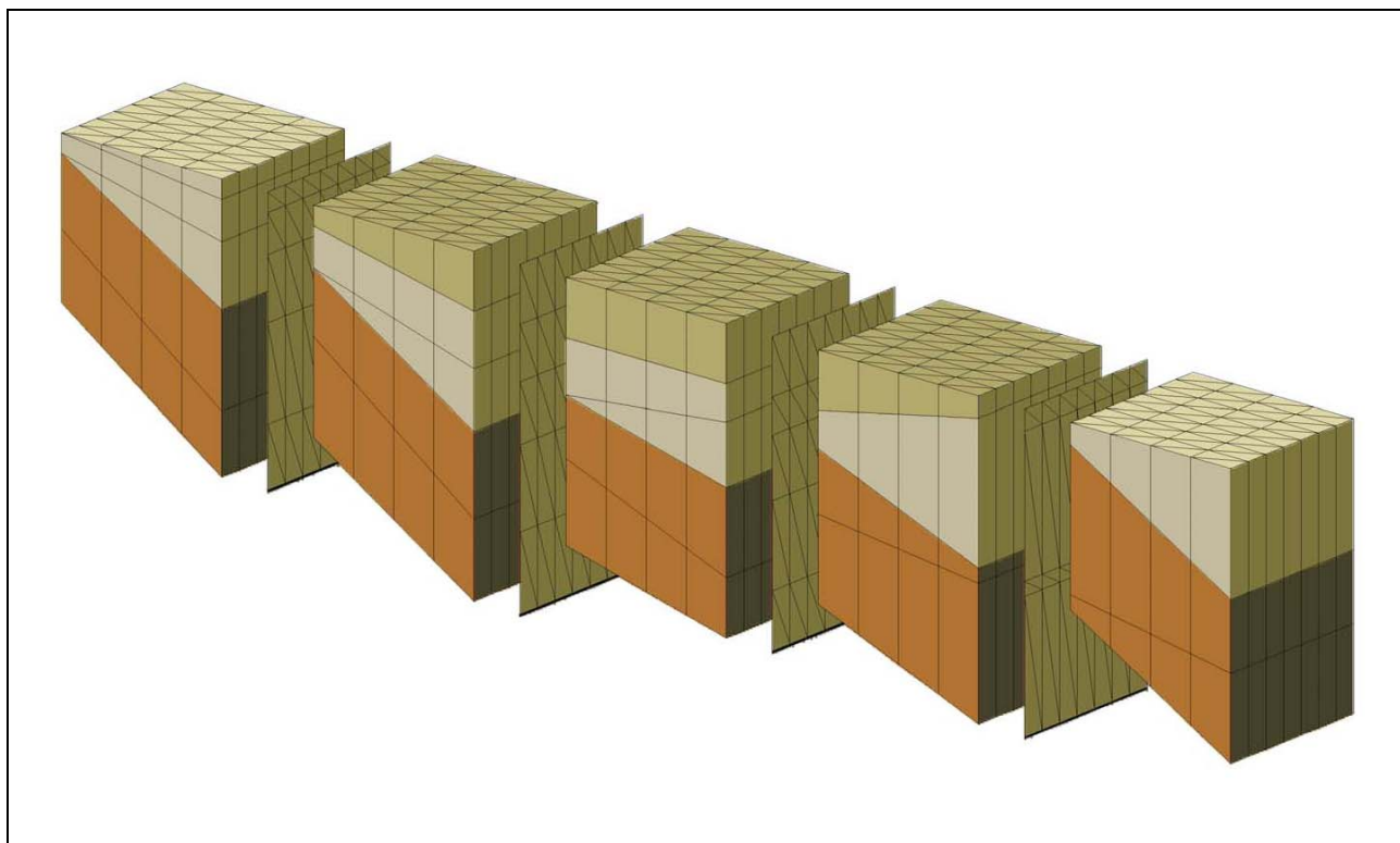
Figure 1-8 Five Hydrogeologic Compartments Offset by Vertical Faults
