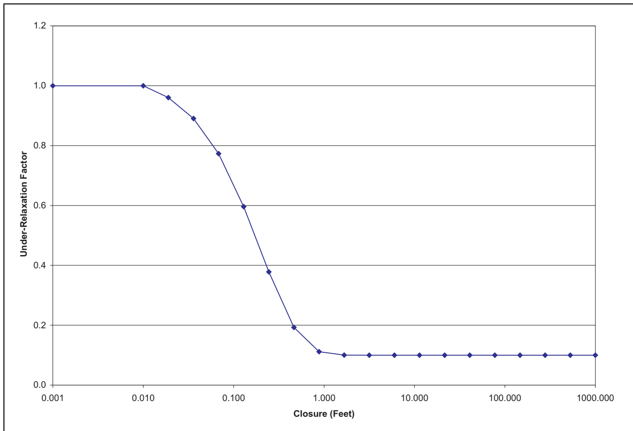
Figure 2-1 Relation Between Under-Relaxation Factor and Iterative Closure
