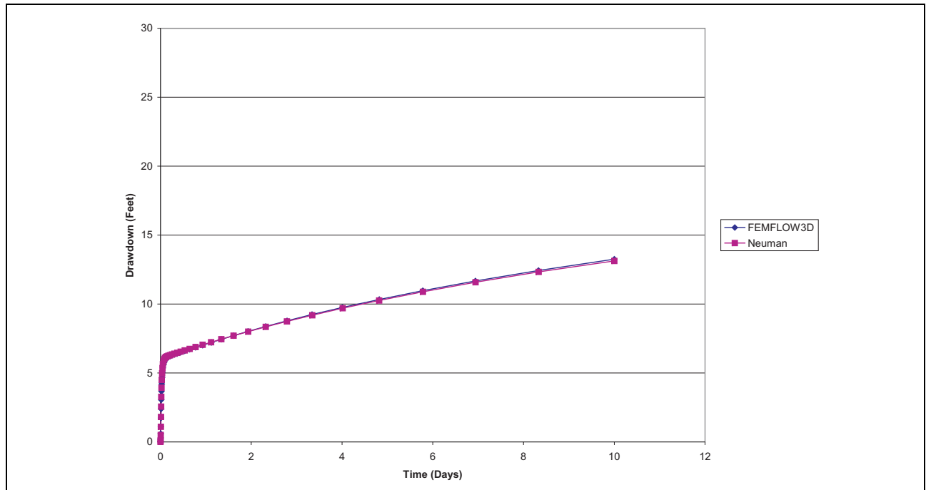
Figure 4-14 Comparison of FEMFLOW3D Simulated Drawdowns With Neuman Solution for Middle Well at a Distance of 400 Feet From Pumping Well
