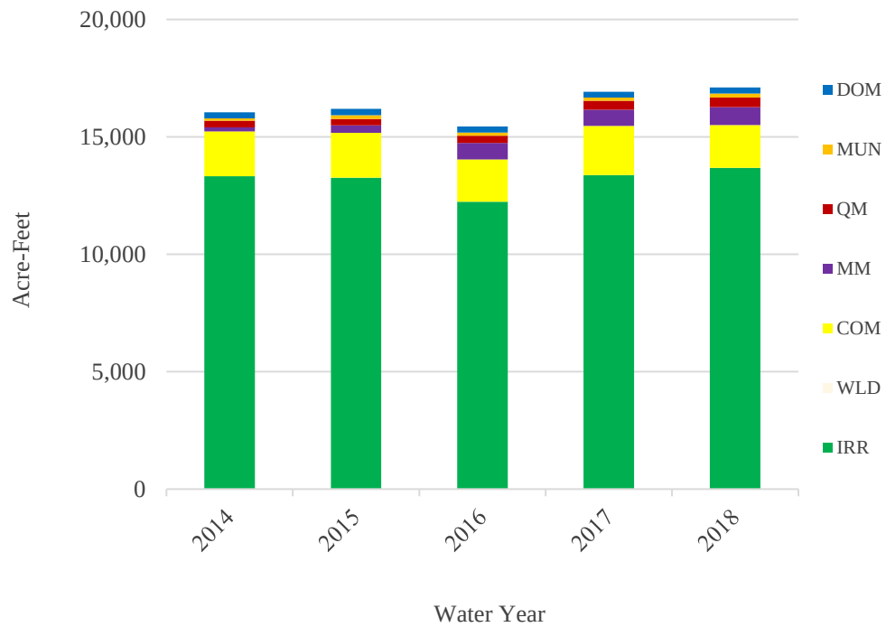
Figure 3. Amargosa Desert historical pumpage by manner of use.
