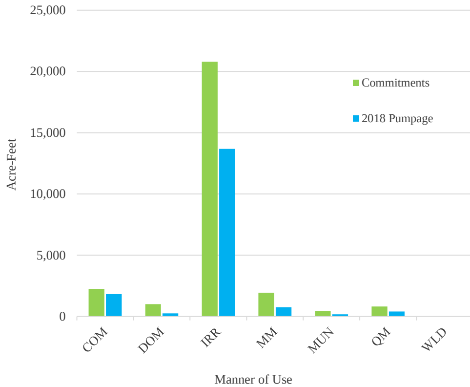
Figure 5. Comparison between 2018 groundwater commitments and estimated pumpage.
