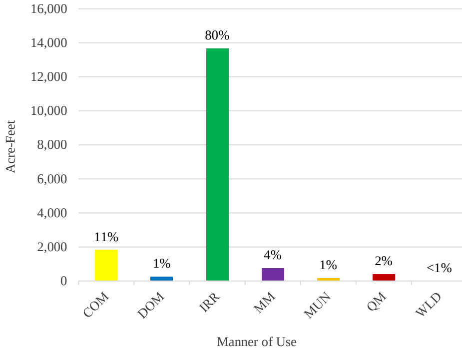
Figure 4. Percentage of 2018 groundwater pumpage by manner of use.
